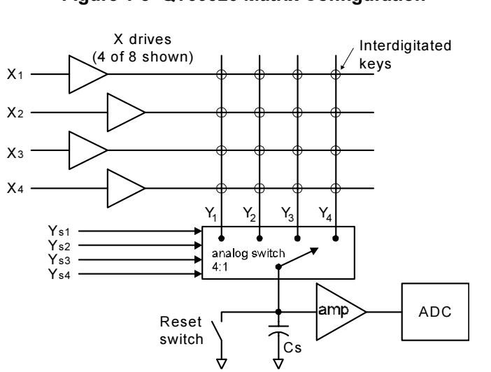
Figure 1-5 QT60320 Matrix Configuration
