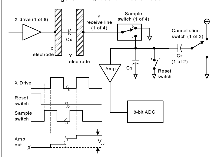
Figure 1-4 QT60320 Circuit Model
